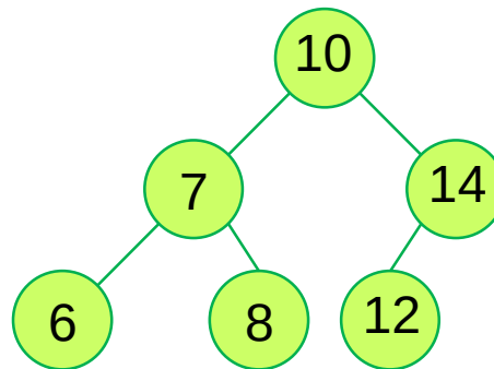
Complete BST
