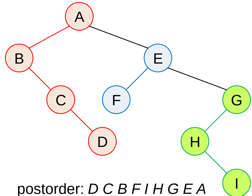
Binary Tree T
