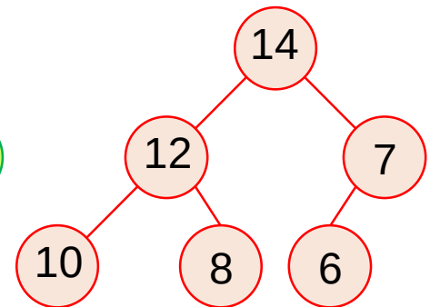
Heap
