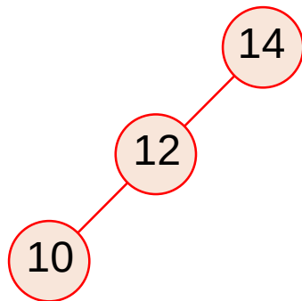
Skewed BST
